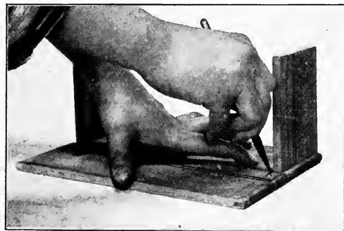
Fig. 291—Transferring Measurement
